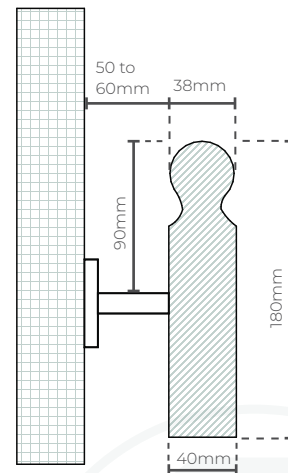
Accessible Handrail
